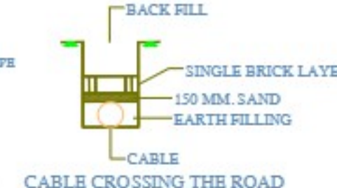
CABLE CROSSING THE ROAD
