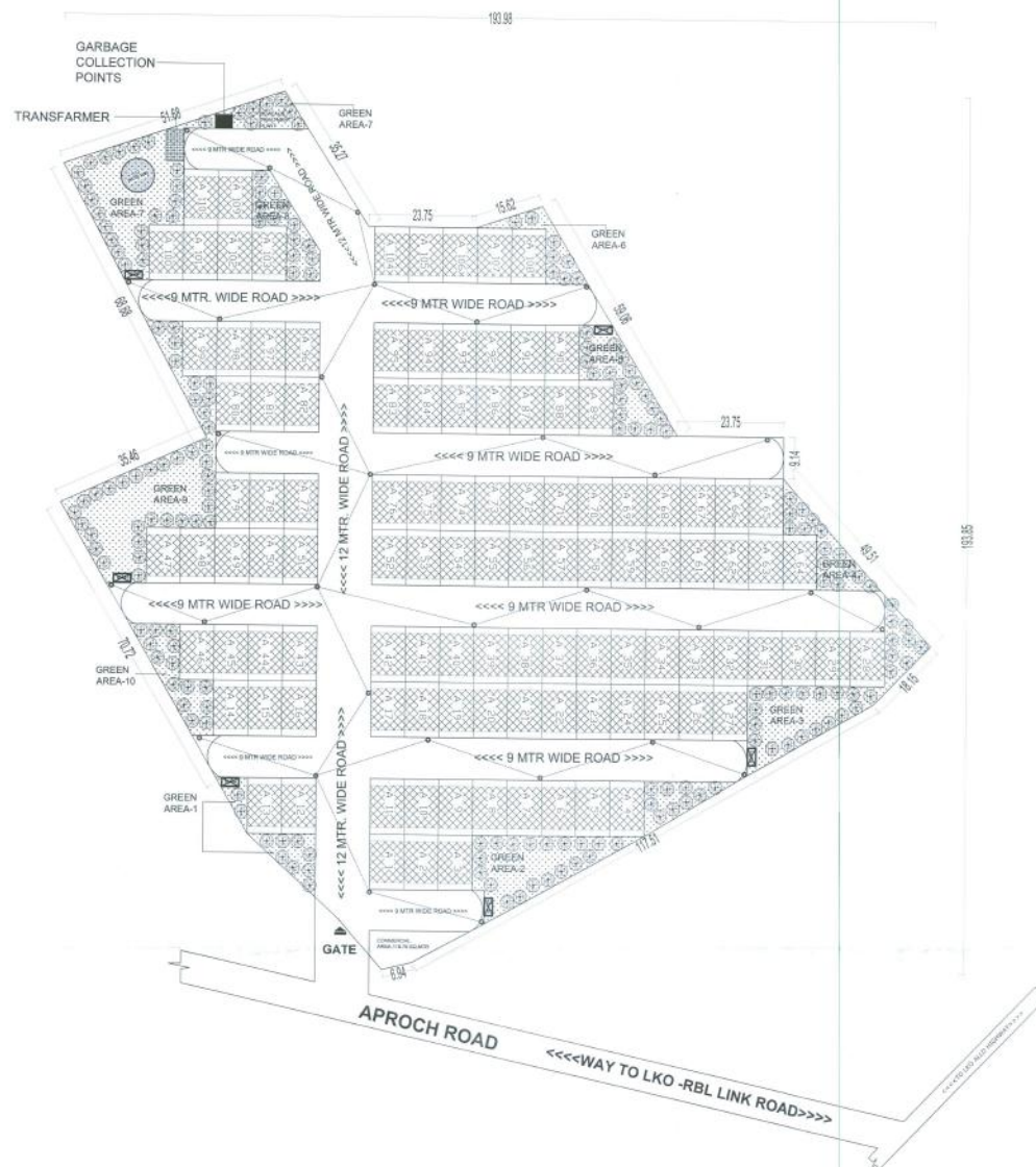
LANDSCAPE AND SERVICES LAYOUT PLAN
