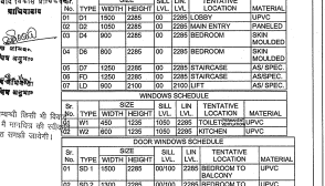
WINDOW SCHEDULE
