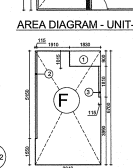
AREA DIAGRAM - UNIT-II
