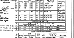
WINDOW SCHEDULE
