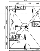
AREA DIAGRAM - UNIT-V
