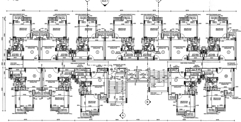
5TH FLOOR PLAN 1:100
