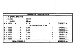
AREA DETAIL OF UNIT PLAN - VI
