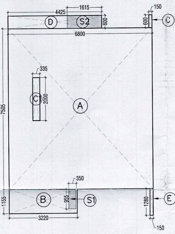
FIRST FLOOR AREA DIAGRAM
