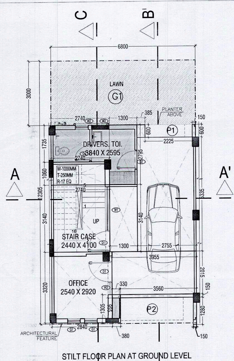
STILT FLOOR PLAN AT GROUND LEVEL
