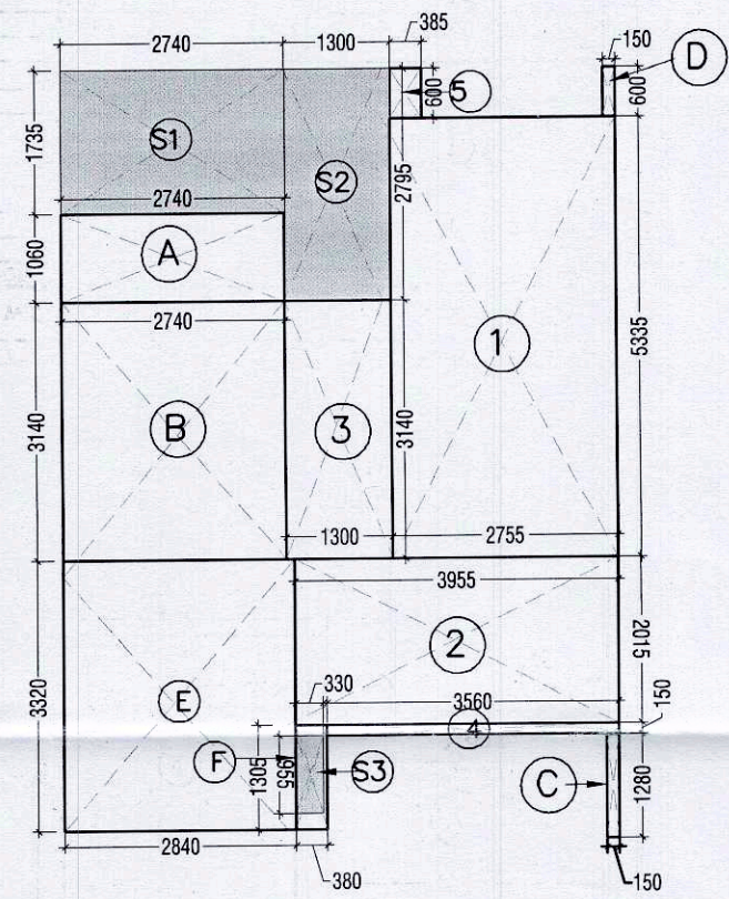
STILT FLOOR AT GROUND LEVEL AREA DIAGRAM
