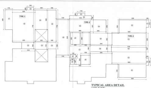
TYPICAL AREA DETAIL (13-14 TH FLOOR FOR BLOCK 1 & 3) Block-1,2,3,4
