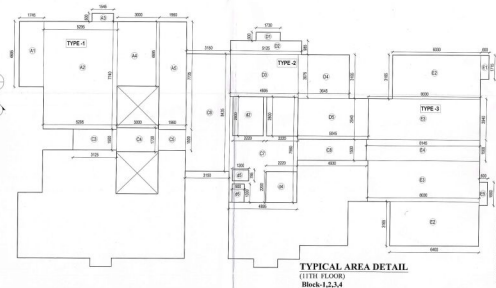
TYPICAL AREA DETAIL (11-12 TH FLOOR FOR BLOCK 1 & 3) Block-1,2,3,4
